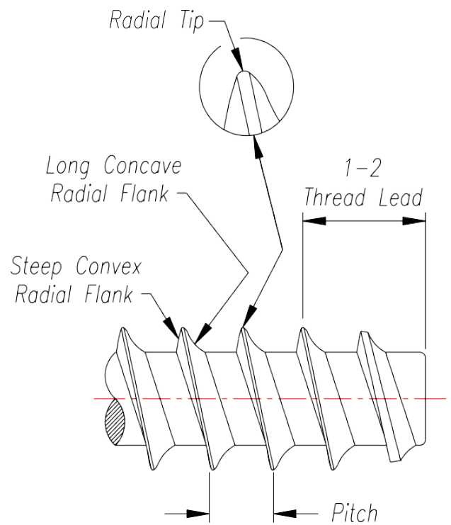
Figure 1: REMFORM® II™ thread profile.
