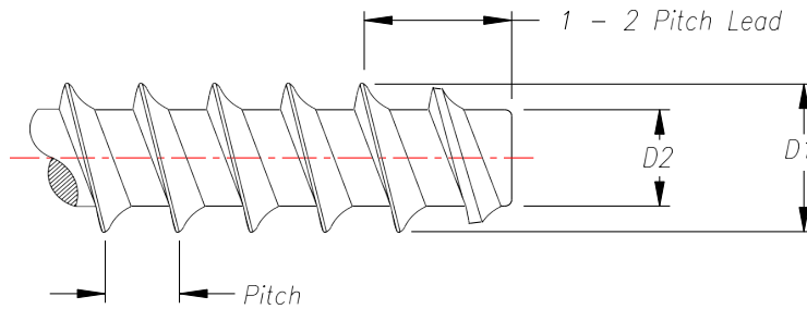
Figure 2: REMFORM® II™ Dimensions.
